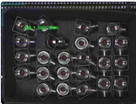
A box of valves. Scorpion sends the valve positions to the robot.
